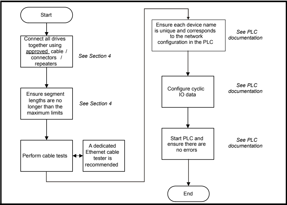
Figure 5-2 SI-PROFINET V2 setup flowchart
