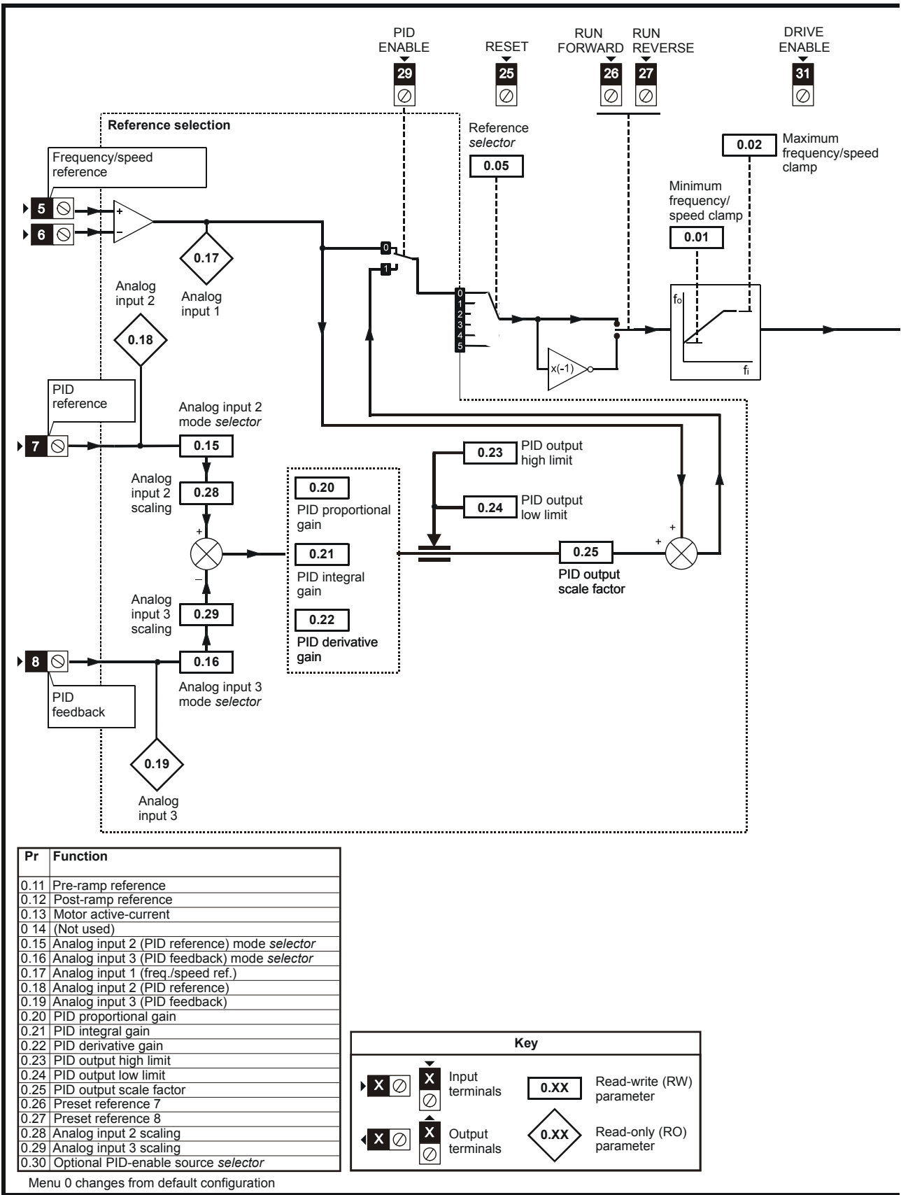
Figure 6-5 Macro 5 PID control logic diagram
