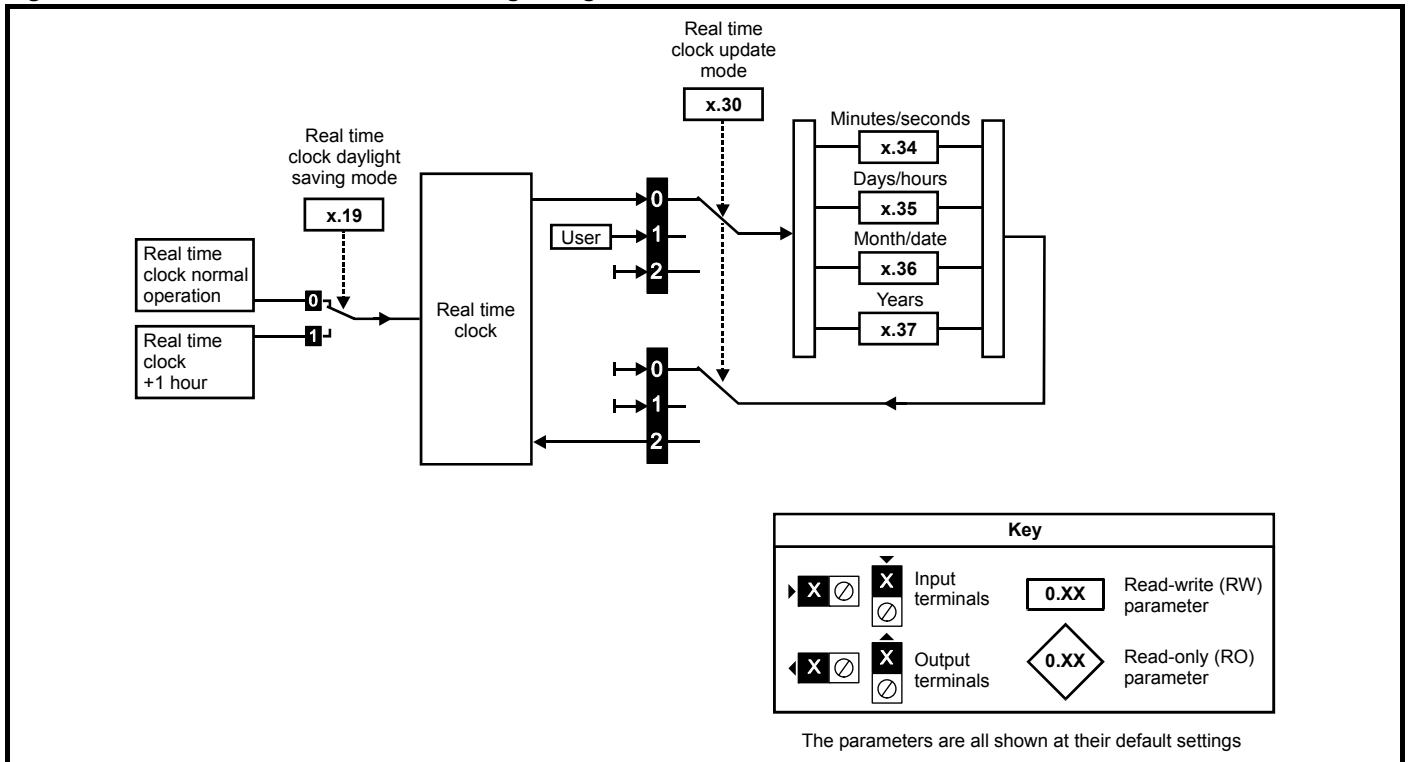
Figure 5-36 SM-I/O Timer real time clock logic diagram
