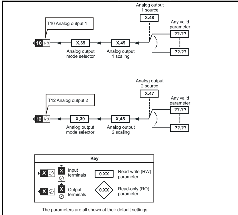
Figure 5-32 SM-I/O 24V Protected analog output logic diagram
