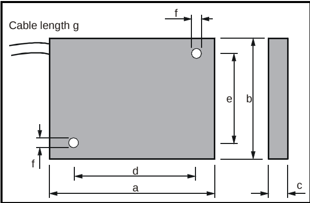
Figure 4-10 Dimensions of the External Braking Resistor
