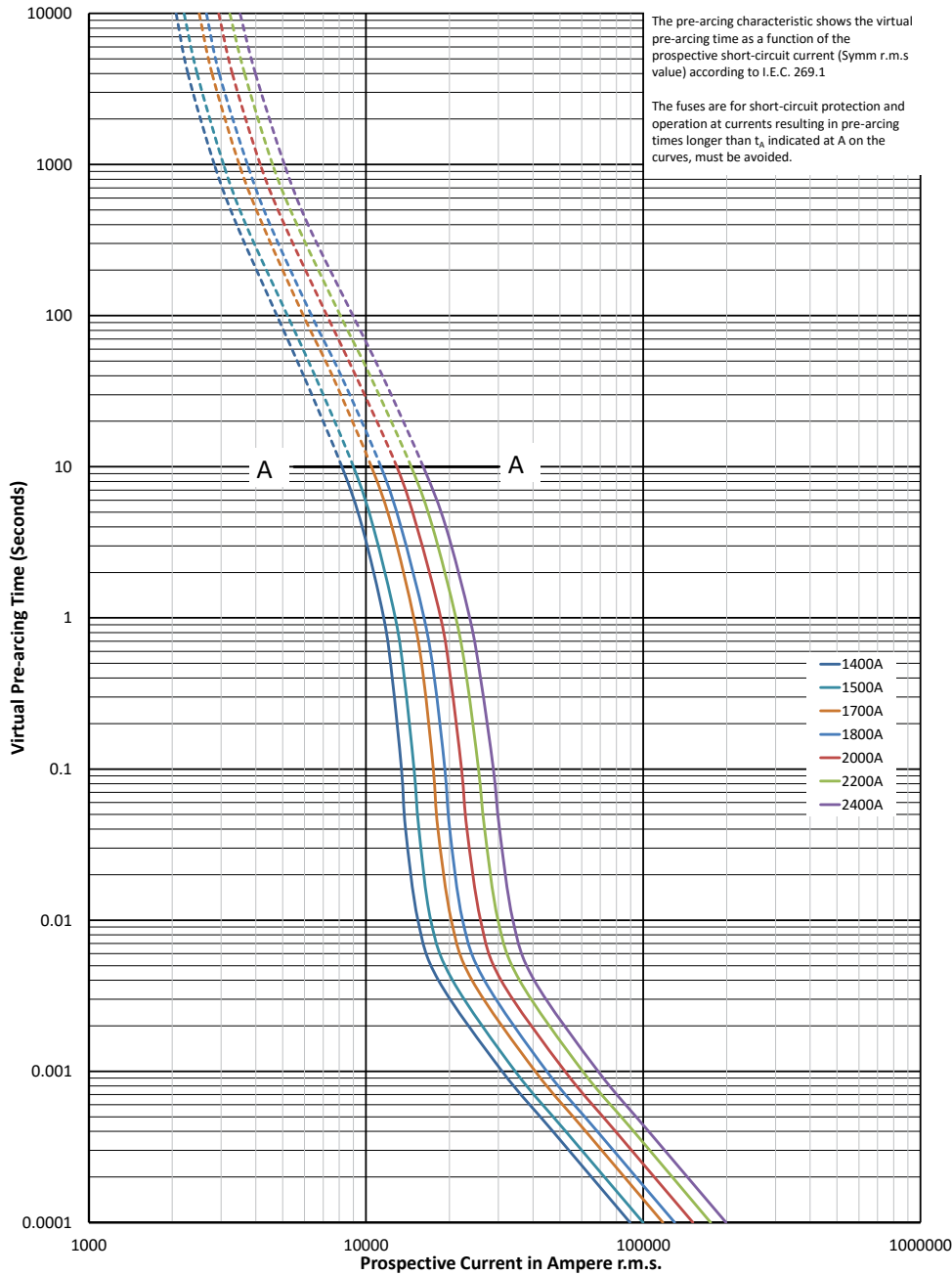
Time-current curve - 1400 A to 2400 A
